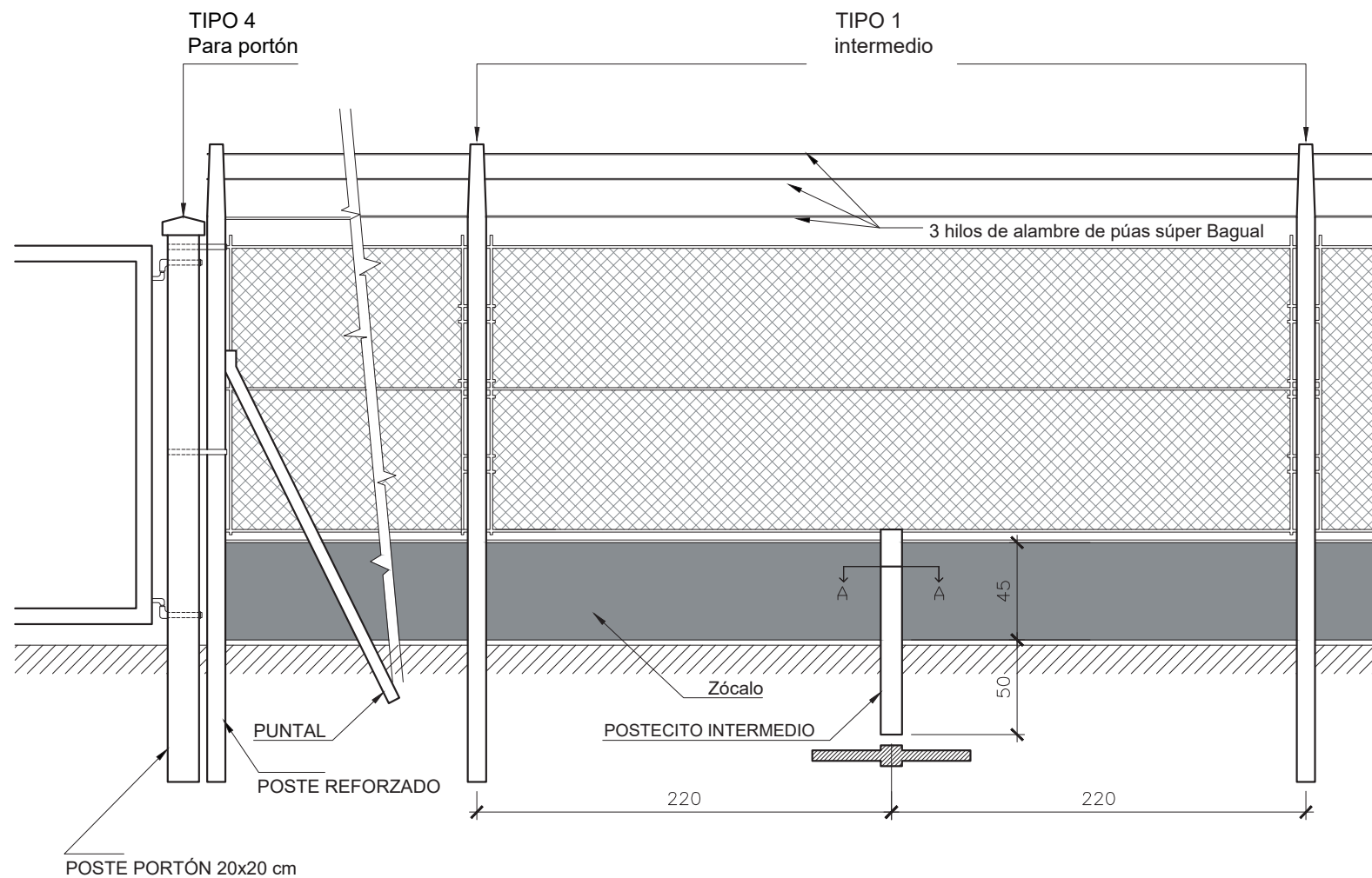
VISTA FRONTAL
